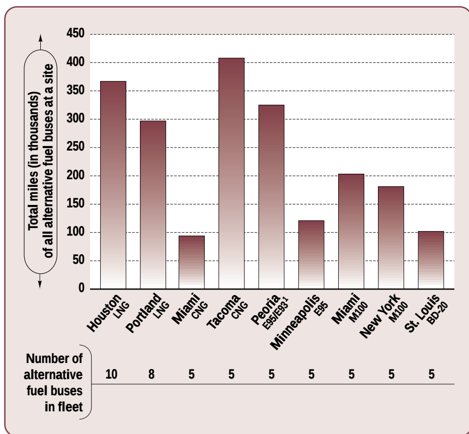
FIGURE 2. Mileage accumulation on the alternative fuel buses by site
