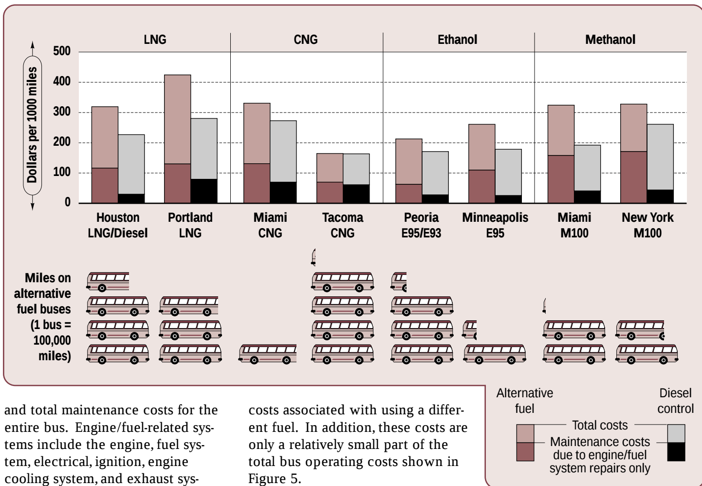
FIGURE 7. Maintenance costs for the buses in the program
