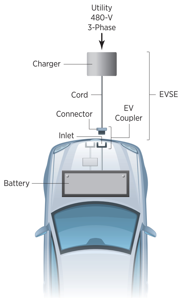
Figure 4. DC fast charging schematic.
