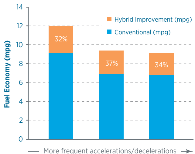
Hybrid vs. Conventional Diesel Package Delivery Trucks
