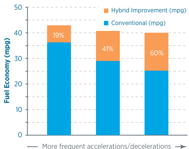
Hybrid vs. Conventional Gasoline Sedans
